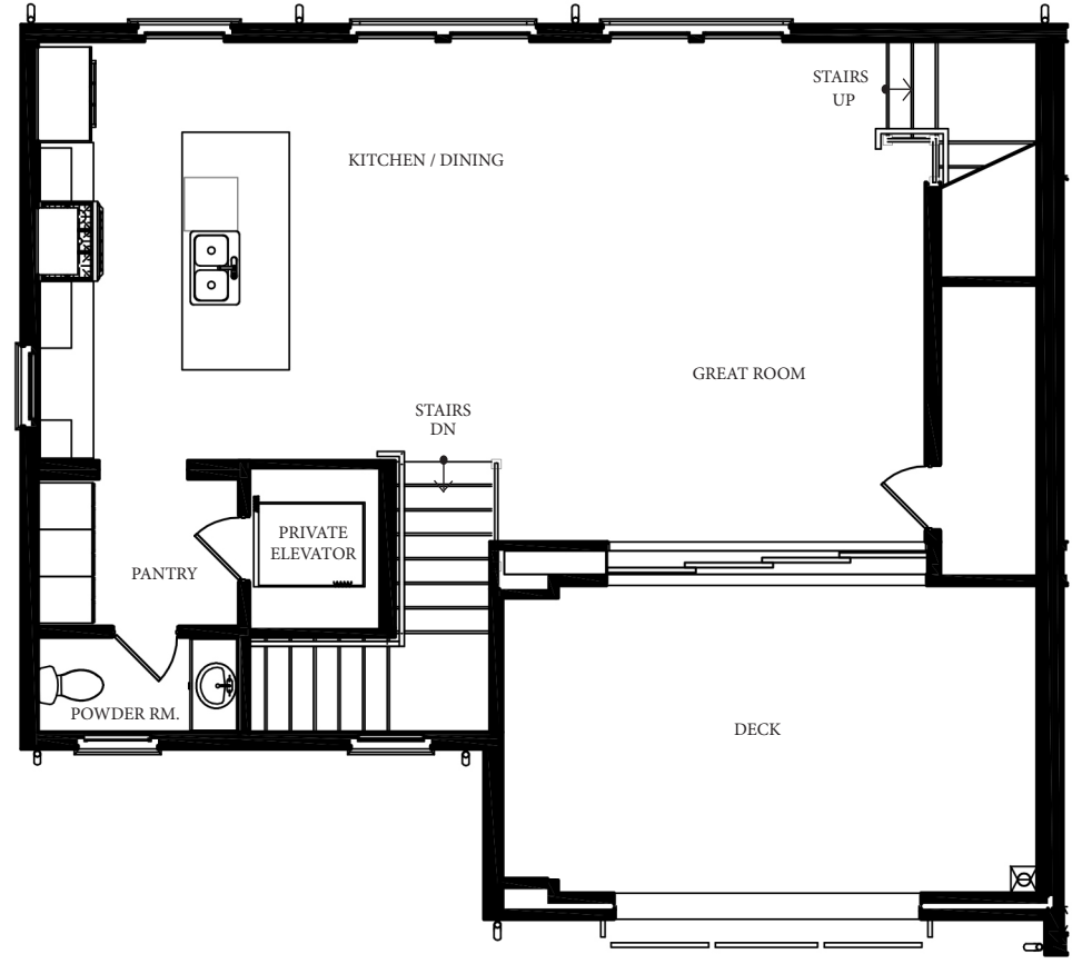
FLOOR 2
